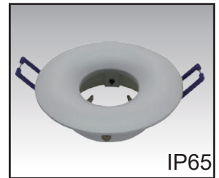
Code: TL9865R Material: ALU. Light Source: MR16/GU10
