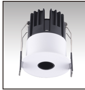
Code: DL-6008 Ø62mm Hole:Ø55mm 8W 200mA
